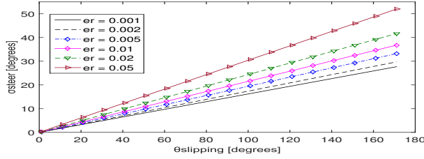
Fig. 3: The required steering wheel accuracy ( \sigma_{steer} ) for given error rate ( e_r ) and slipping angle ( \theta_{slipping} ) is plotted.
