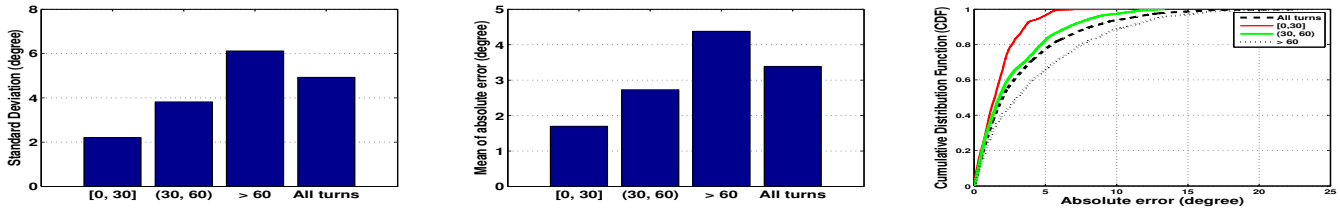
(a) The comparison of the standard deviation of the true error for the turns with different ranges of steering wheel angle. (b) The comparison of the mean absolute error for the turns with different ranges of steering wheel angle. (c) The cumulative distribution function of absolute error for the turns with different ranges of steering wheel angle.
