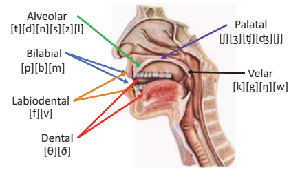
Figure 3: Place of articulation and corresponding consonants.
