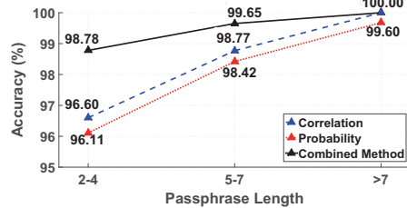
Figure 18: Accuracy under different lengths of passphrase.
