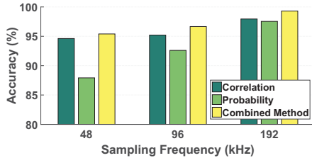
Figure 20: Accuracy under different sampling frequencies.
