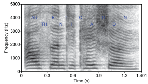
Figure 9: Example of segmented phonemes.
