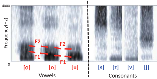
Figure 8: Example: spectrogram of phonemes.
