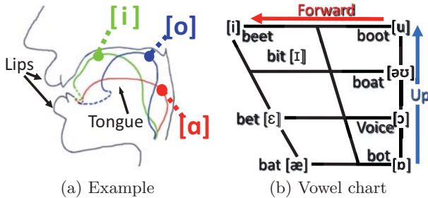
Figure 2: Tongue positions of English vowels within the oral cavity, and the vowel chart.
