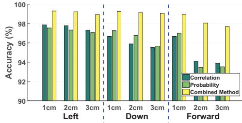
Figure 23: Accuracy under different degree of phone displacement.
