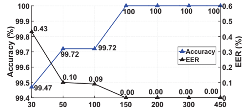
Figure 17: Replace Attacks: EER and Accuracy of Combined method under different distances.
