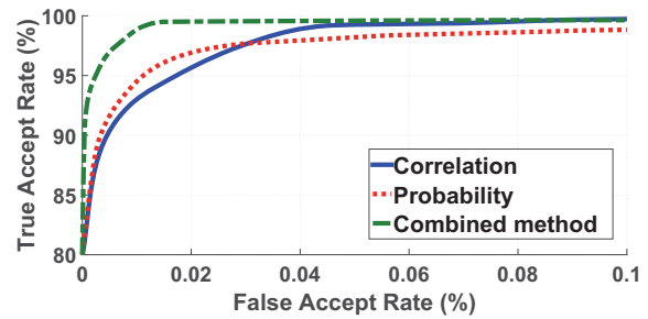
Figure 13: Playback Attacks: ROC curves under different methods.
