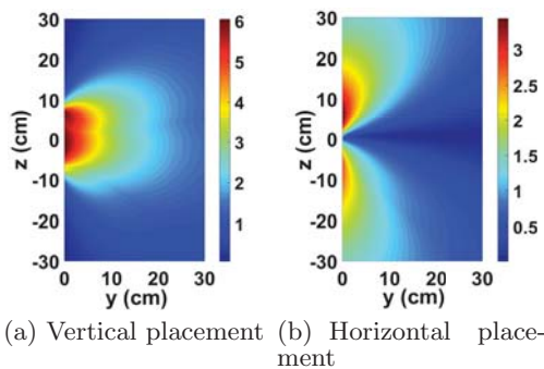
Figure 27: The achievable TDoA range under both vertical and horizontal placements.
