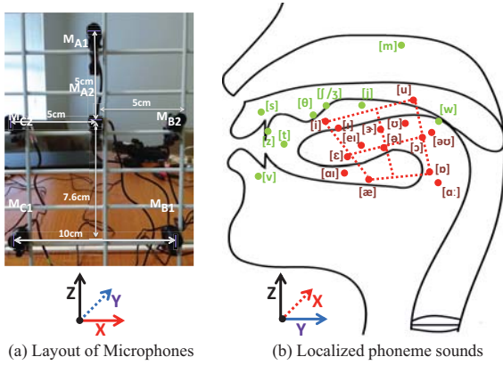
Figure 5: Phonemes localization using microphone array.
